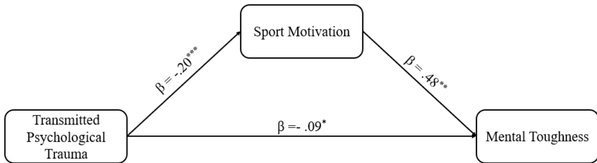
Figure 1. Mediation model illustrating the indirect effect of transmitted psychological trauma on mental toughness through sport motivation
