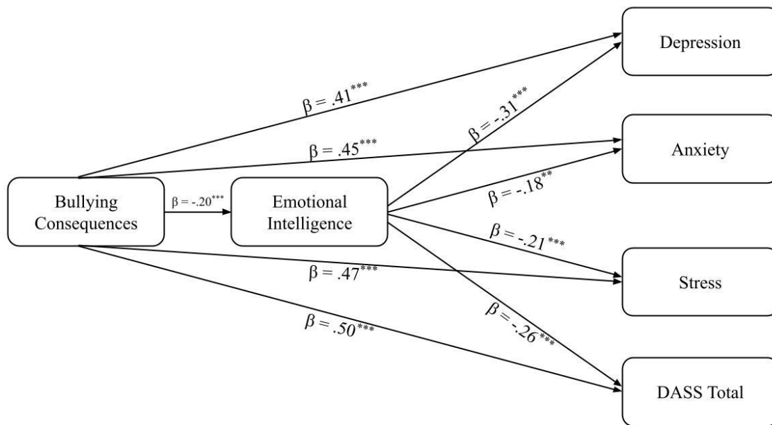
Figure 1. Mediation model illustrating the effects of bullying consequences on DASS depression, anxiety, stress and total scores through emotional intelligence
